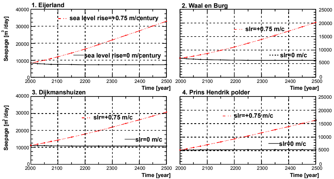
Figure 6: Seepage (in m^3/day ) through the top layer at -0.75 m N.A.P. of the four polder areas as a function of 500 years.
