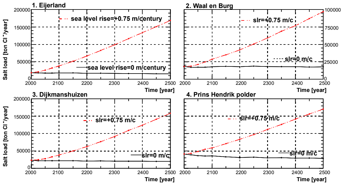
Figure 7: Salt load (in ton Cl - /year) through the top layer at -0.75 m N.A.P. of the four polder areas as a function of 500 years.
