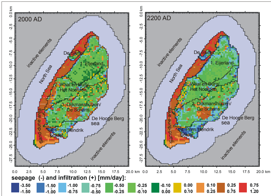
Figure 3: Seepage through the top layer at -0.75 m N.A.P. for the years 2000 and 2200 AD. Sea level rise is 0.75 meter per century.
