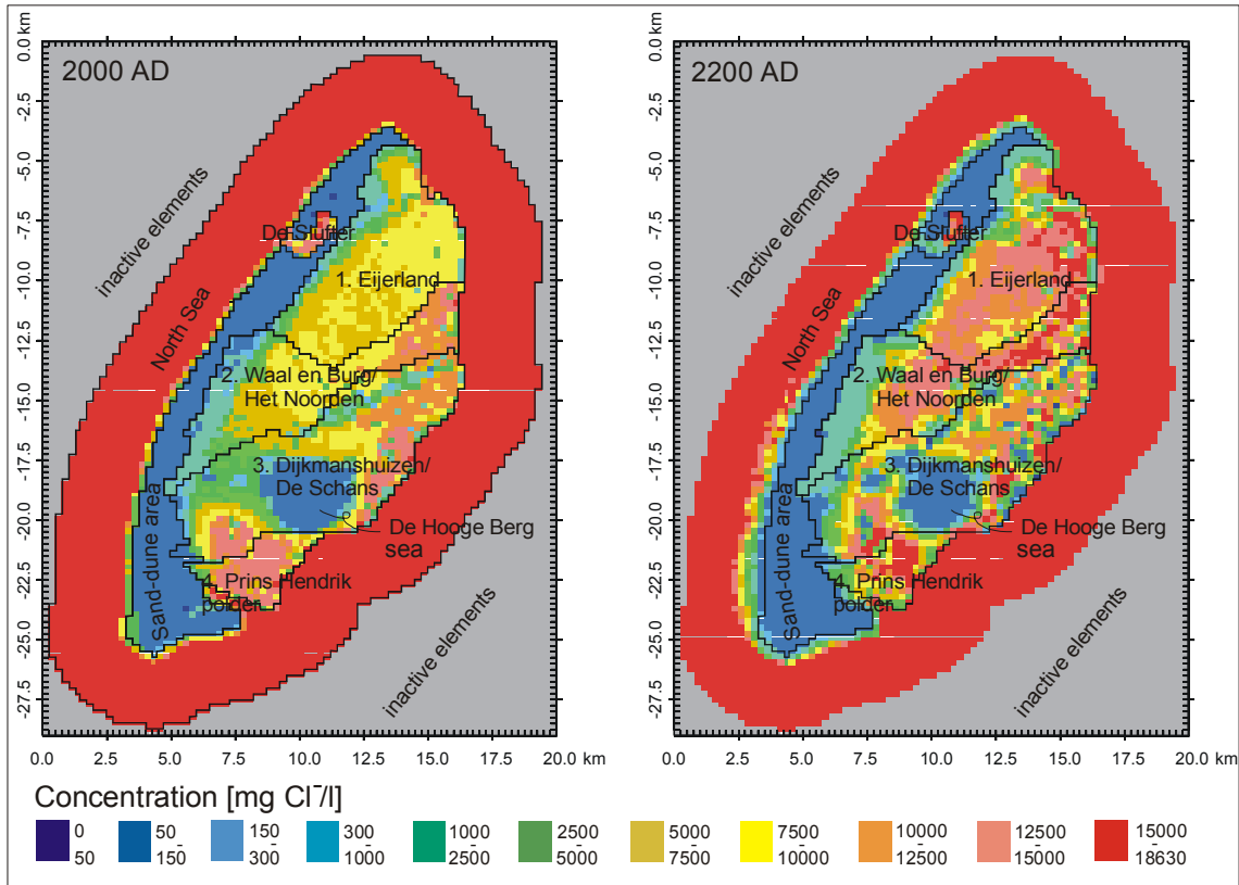
Figure 2: Chloride concentration in the top layer at -0.75 m N.A.P. for the years 2000 and 2200 AD. No sea level rise is simulated.
