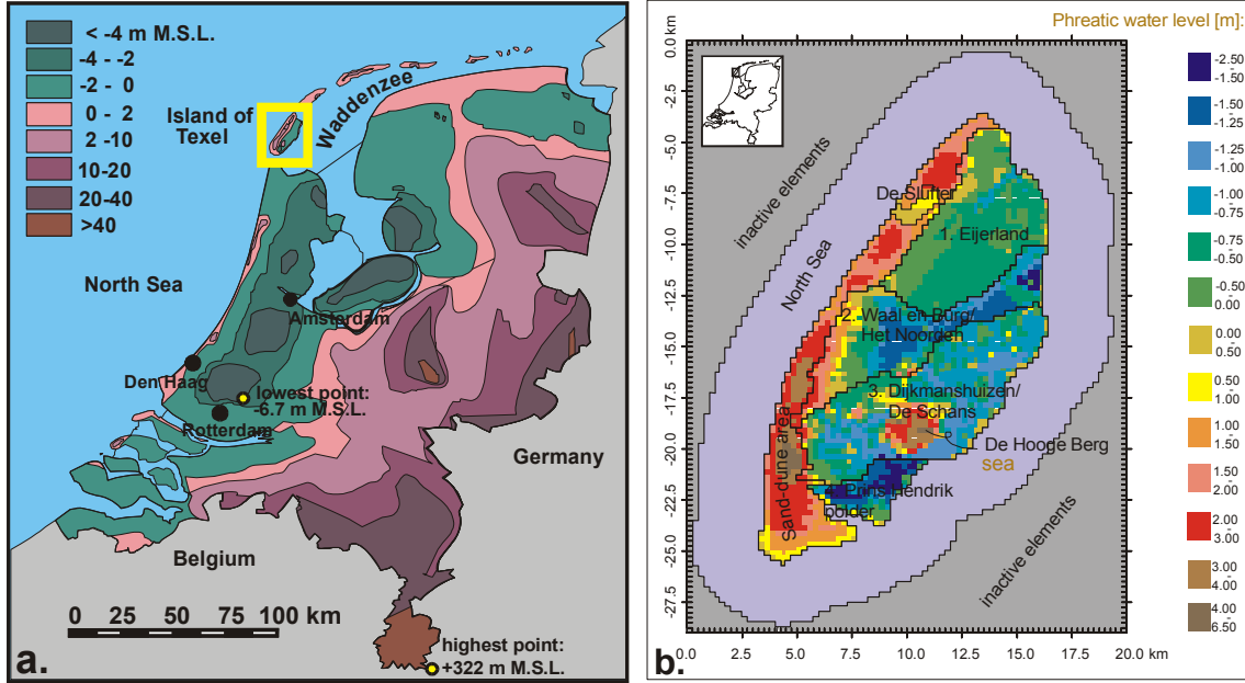
Figure 1: a. map of The Netherlands: position of the island of Texel and ground surface of the Netherlands; b. map of the island of Texel: position of the four polder areas and sand-dune area as well as phreatic water level in the top aquifer at -0.75 m N.A.P.
