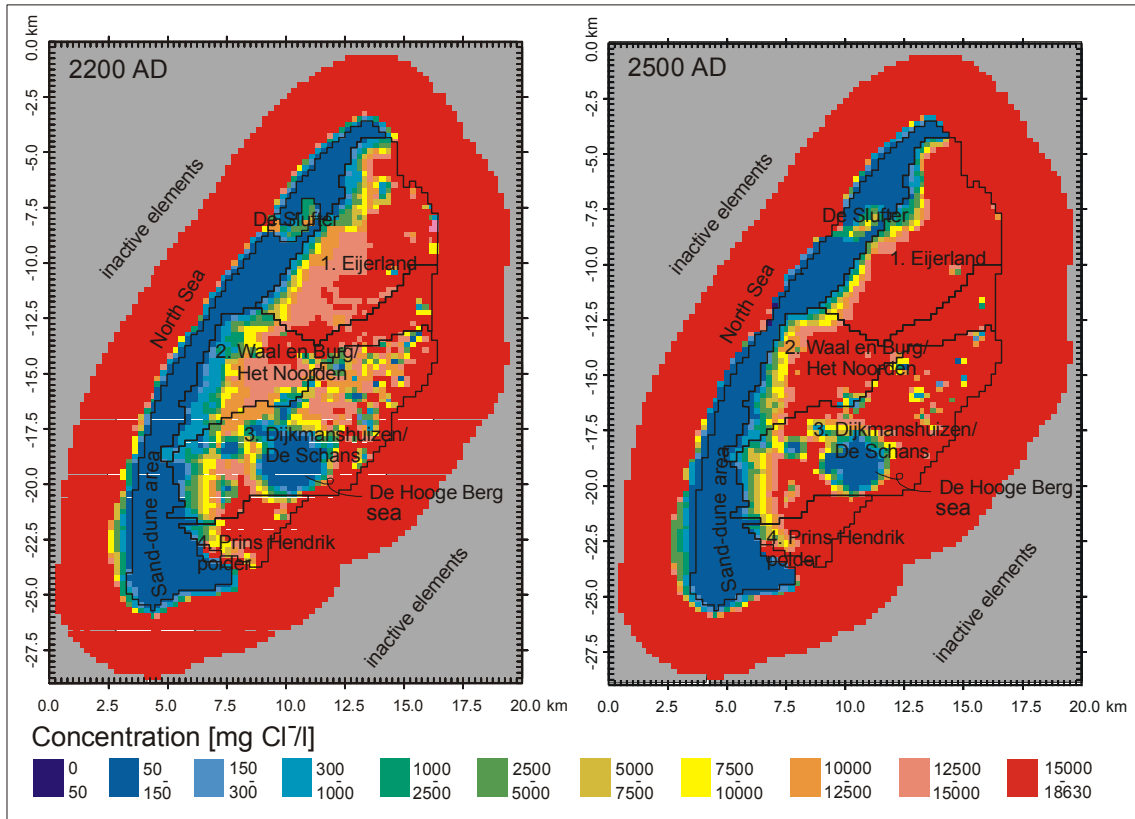
Figure 5: Chloride concentration in the top layer at -0.75 m N.A.P. for the years 2200 and 2500 AD. Sea level rise is 0.75 m per century.
