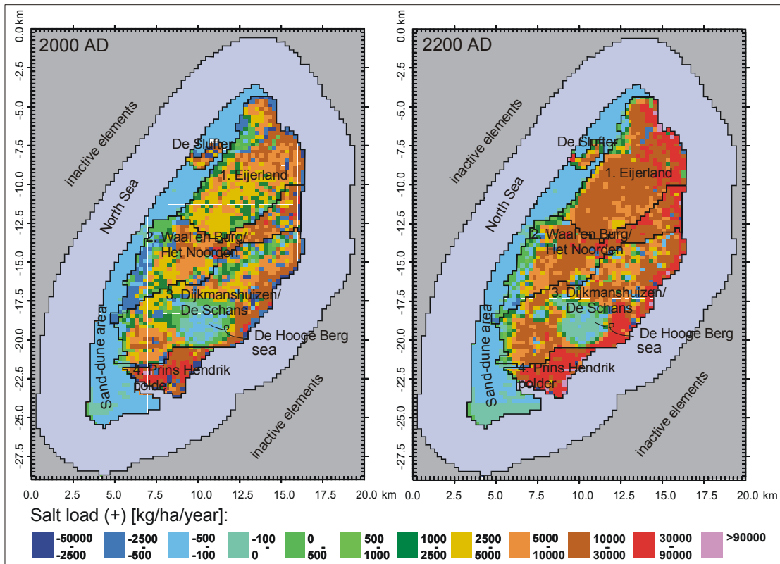
Figure 4: Salt load (in kg/ha/year) in the top layer at -0.75 m N.A.P. for the years 2000 and 2200 AD. Sea level rise is 0.75 meter per century.
